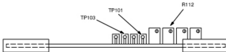
Illustration 5-18: Low Level Set Adjustment
