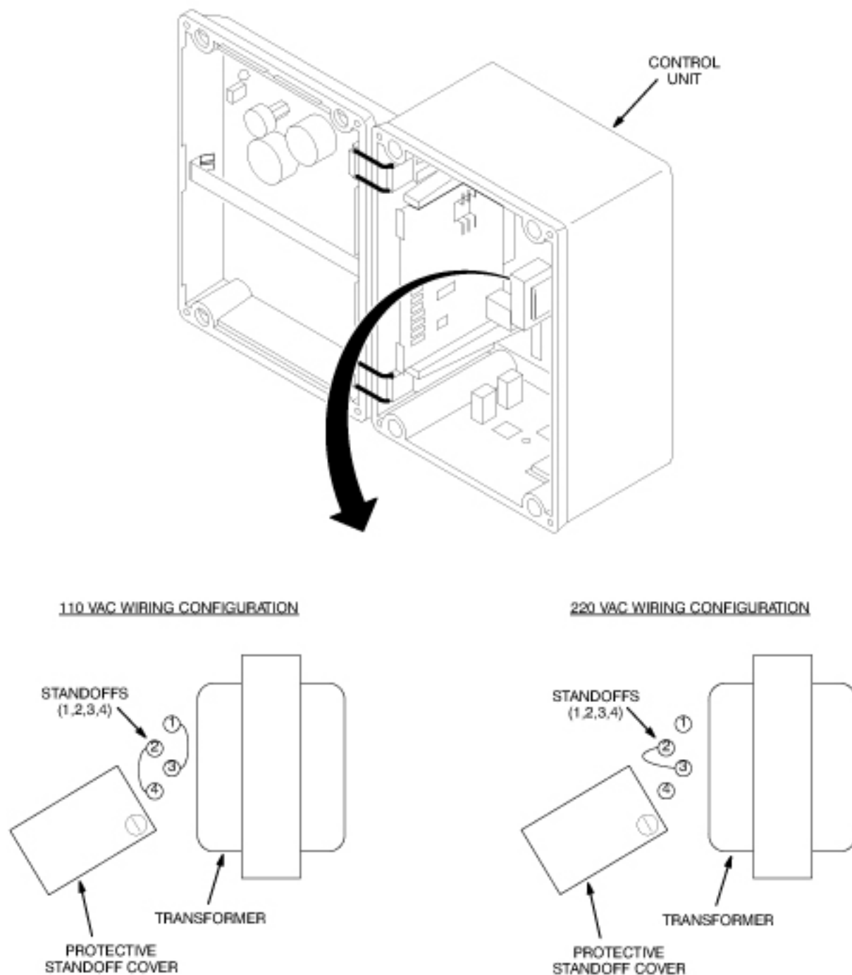
Illustration 4-9: Transformer Configuration
