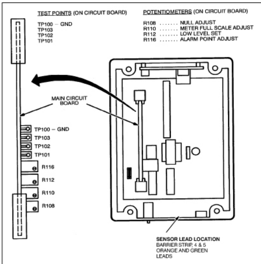
Illustration 5-9: Low Level Set Adjustment
